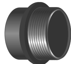
Male Adapter Spg x MIPT - ABS DWV for Aquatica bath wastes with Sch40 hub outlet. Thread: 1 1/2" NPSM (1 1/2" IPS)
