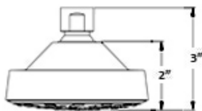
SH0160100 / SH0160400
