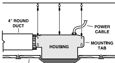
SUSPENDED CEILINGS Housing hung with wires - 3-point mount.
