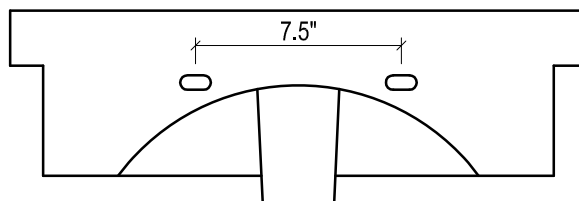
BACK VIEW
