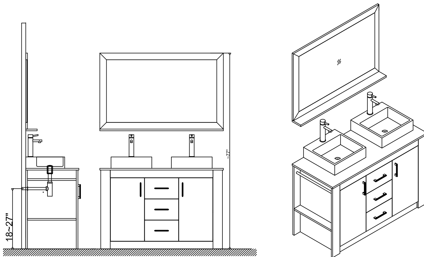
3. Basin
