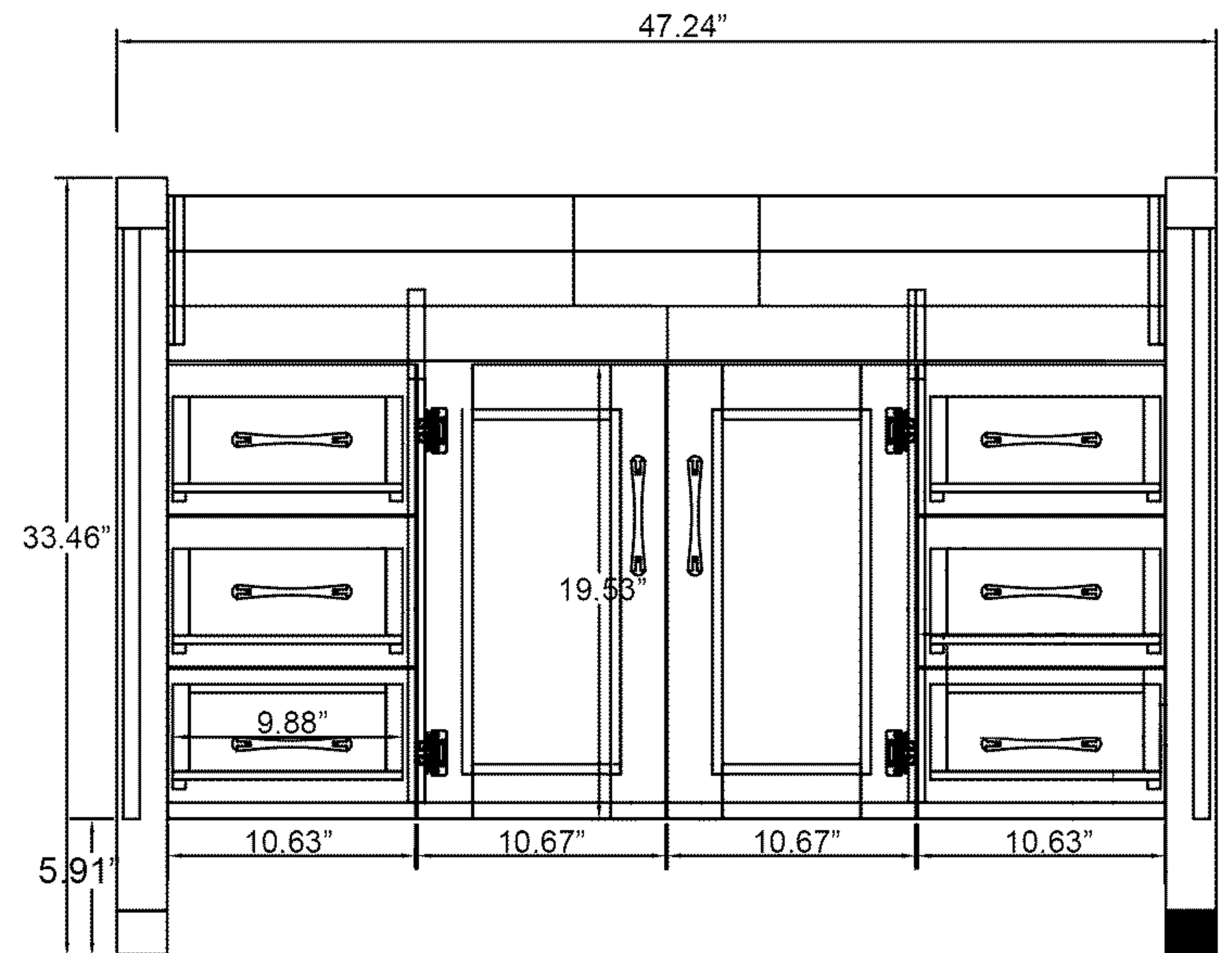
Front View
