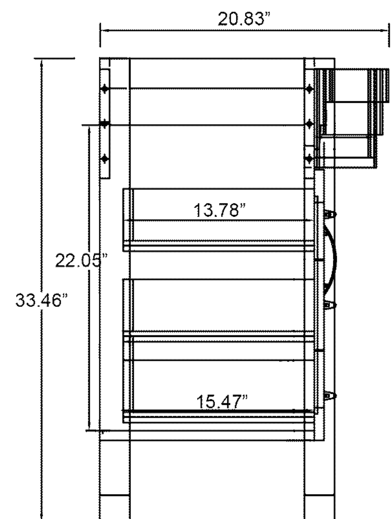
Side View
