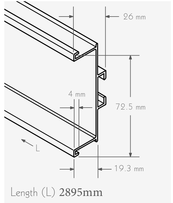
C-PROFILE
