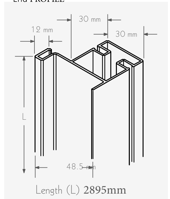
End PROFILE
