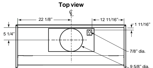
MODEL RMIP45 WITH 331H, 332H, 335 OR 336 BLOWER (Vertical Outlet)
