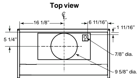
MODEL RMIP33 WITH 331H, 332H, 335 OR 336 BLOWER (Vertical Outlet)
