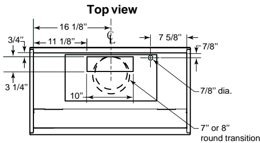
MODEL RMIP33 WITH 331H, 332H, 335 OR 336 BLOWER (Vertical Outlet)
