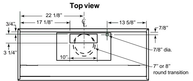
MODEL RMIP45 WITH 331H, 332H, 335 OR 336 BLOWER (Vertical Outlet)
