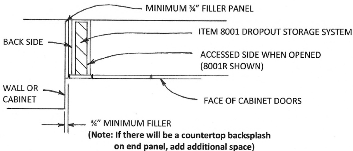
PLAN VIEW
